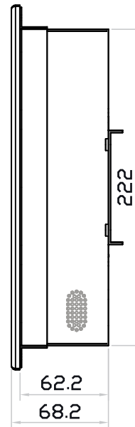
Left-side View
