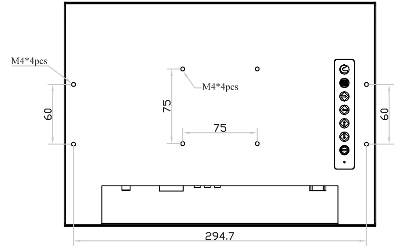
Rear View
