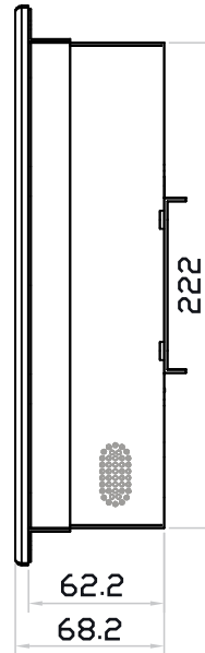
Left-side View
