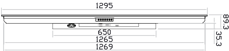
Bottom View
