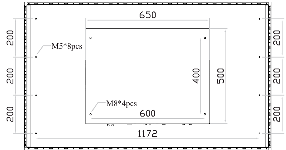
Rear View
