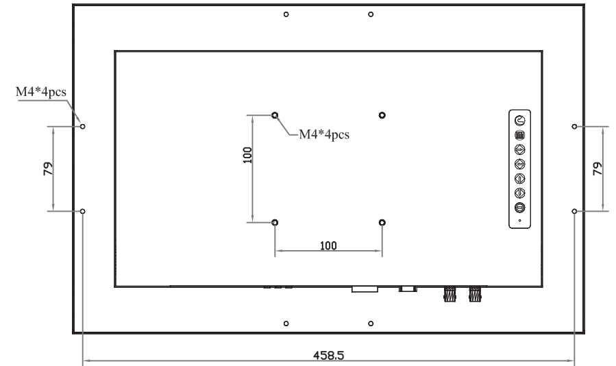
Rear View
