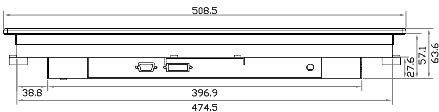
Bottom View
