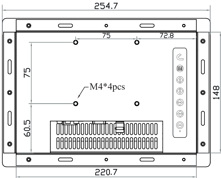
Rear View
