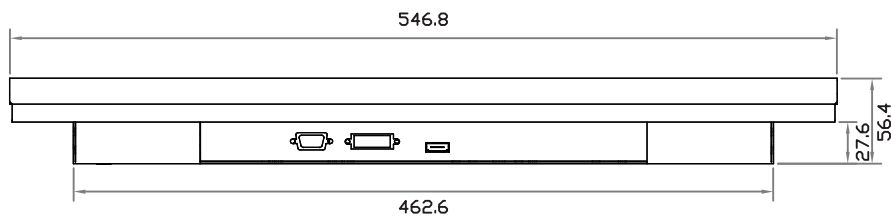
Bottom View
