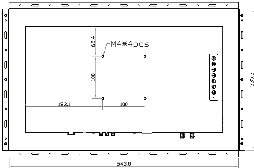
Rear View
