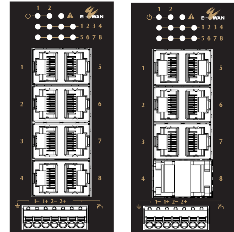
TF100(H)-0800 TG100(H)-0800
