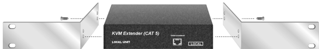
Figure 20 SDBR1 Mounting Kit
