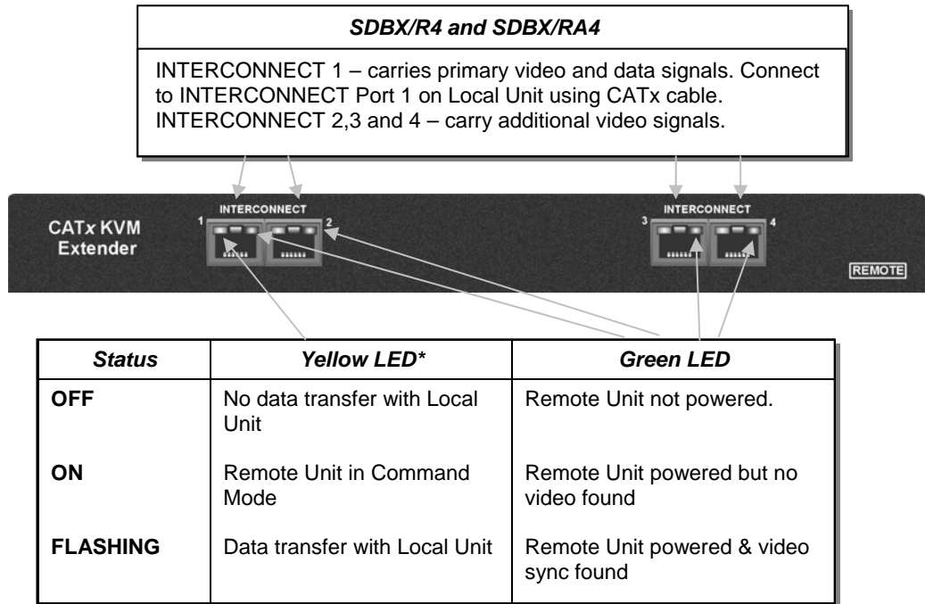
Figure 4 Quad Head Remote Unit – rear view
