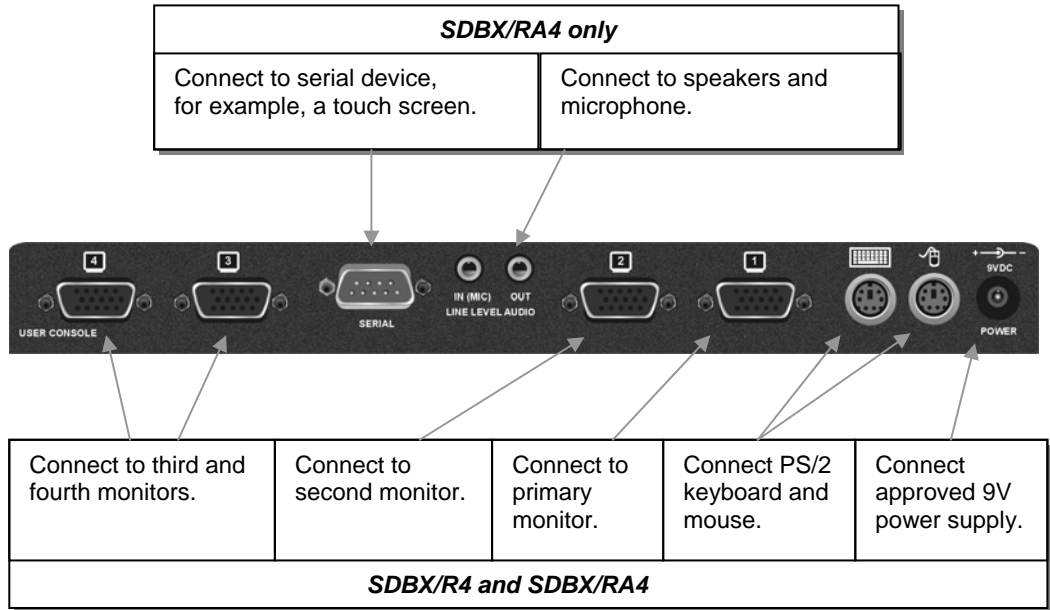
Figure 4 Quad Head Remote Unit – rear view
