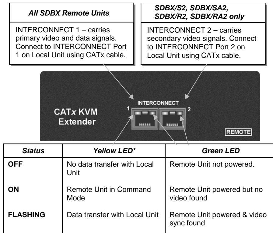
Figure 2 Single/Dual Head Remote Unit – rear view
