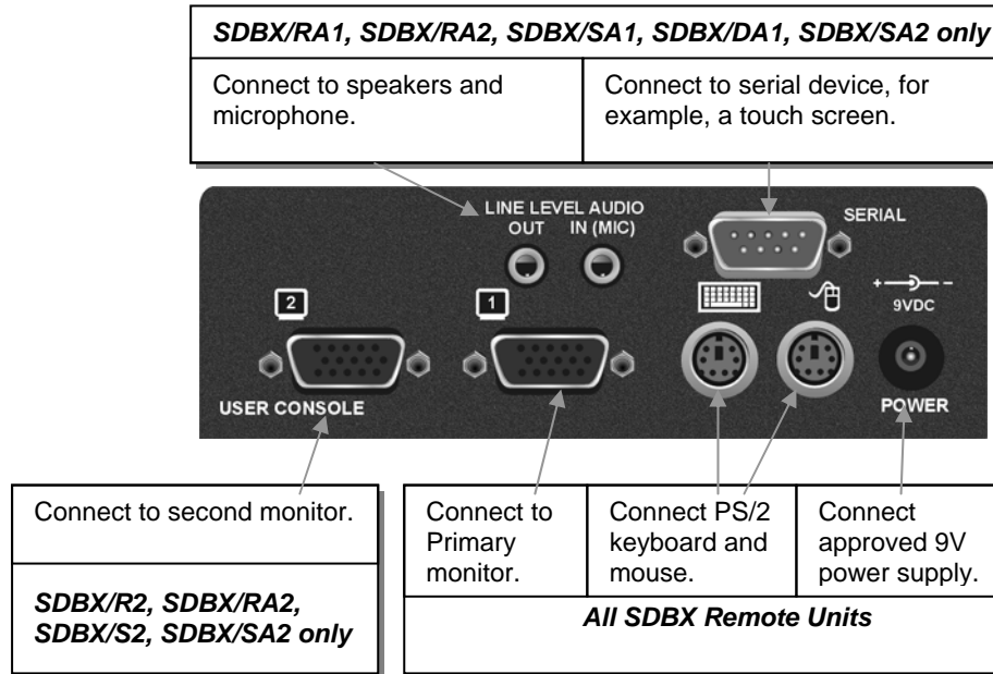
Figure 2 Single/Dual Head Remote Unit – rear view
