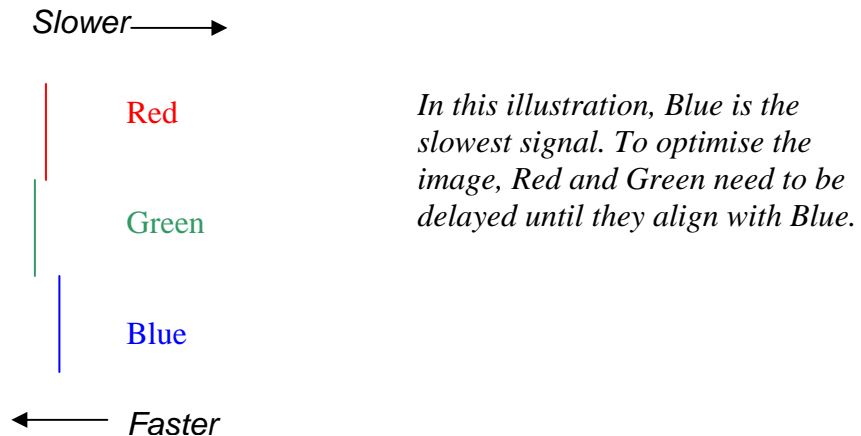
Figure 13 Illustration of skew and appearance on test card
