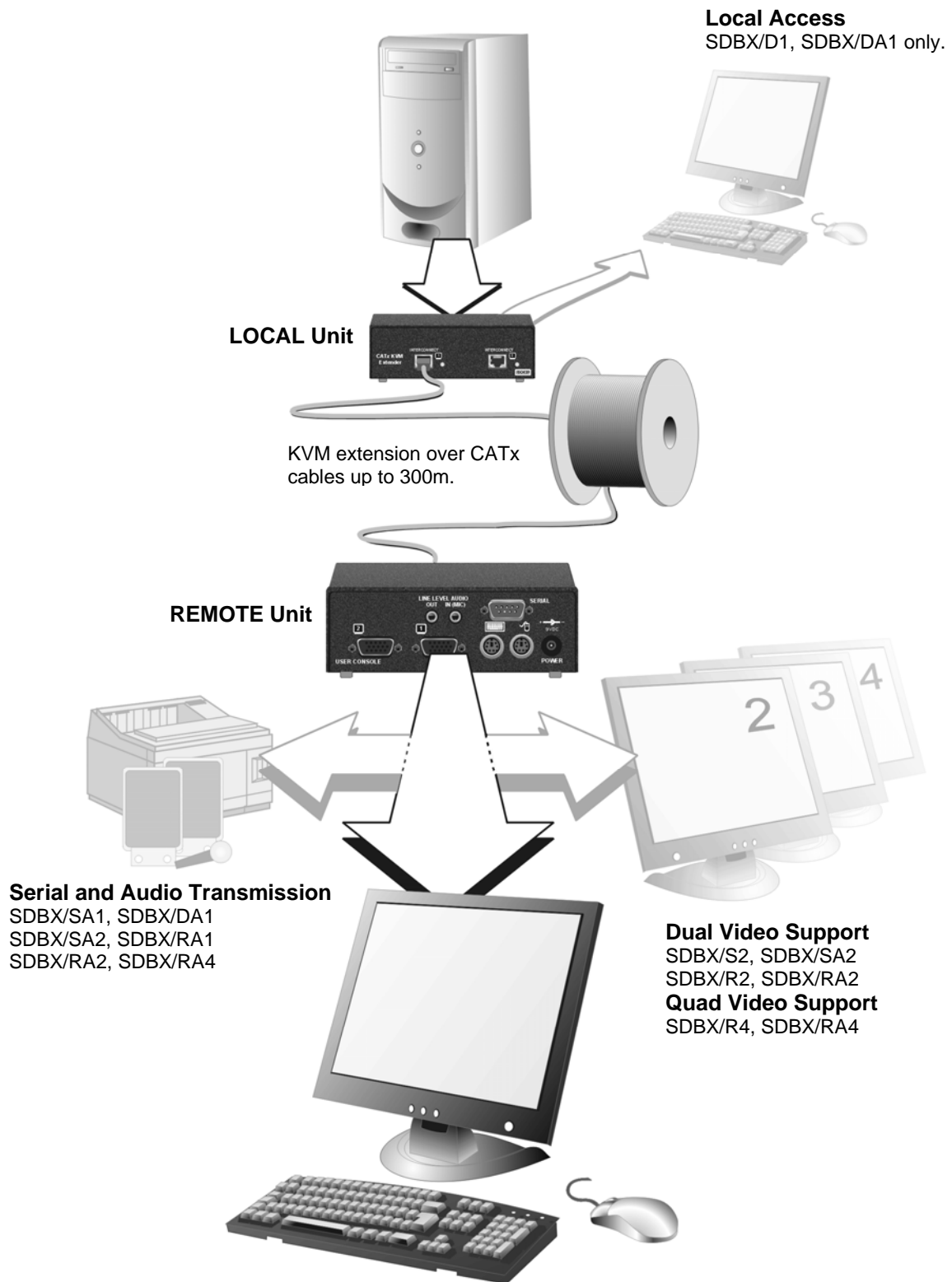
Figure 1 SDBX KVM extender system
